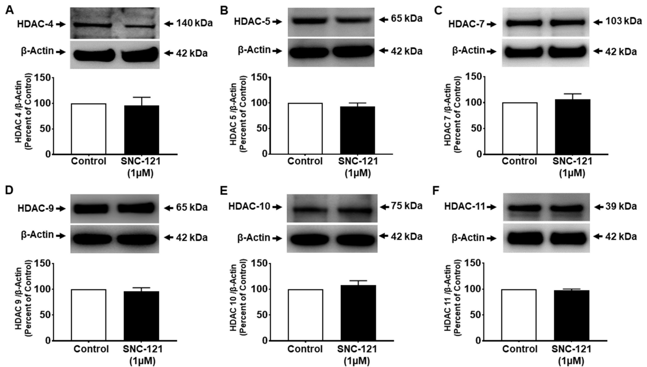
FIGURE 8. Effects of SNC-121 on the expression of (A) HDAC 4, (B) HDAC 5, (C) HDAC 7, (D) HDAC 9, (E) HDAC 10, and (F) HDAC 11 in ONH astrocytes. Cell lysates (20 μg) were analyzed by Western blotting using anti-HDAC 4, anti-HDAC 5, anti-HDAC 7, anti-HDAC 9, anti-HDAC 10, anti-HDAC 11, or anti-β-actin antibodies. The band intensities were measured using chemiluminescent reagent and Versadoc imaging system. Data are expressed as mean ± SE, n = 4-10 . Protein bands shown are representative of at least 4 independent experiments.
