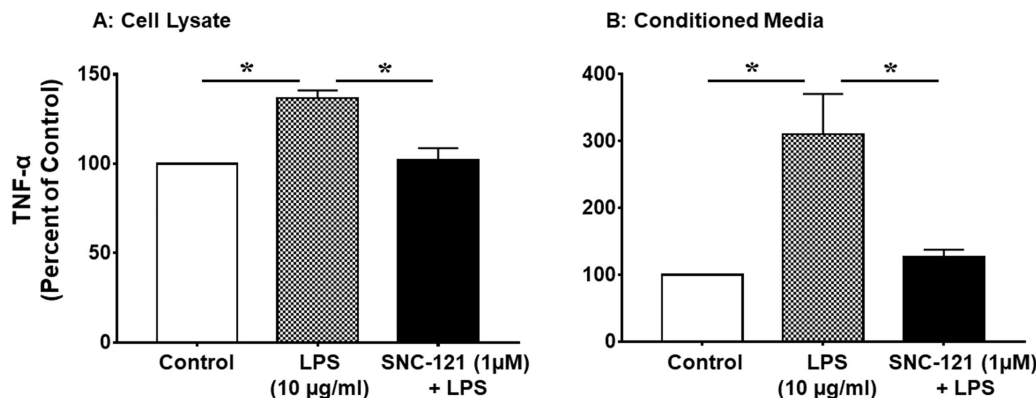
FIGURE 9. Effects of SNC-121 on LPS-induced TNF-α production in (A) cell lysates and (B) conditioned media of ONH astrocytes. Cells were starved in serum-free astrocyte basal medium for 16 hours followed by treatment with SNC-121 (1 μM) for 24 hours followed by treatment with LPS (10 μg/mL) for 6 hours at 37°C. The equivalent amounts of cell lysate (50 μL) and conditioned media (100 μL) were analyzed for TNF-α by ELISA as per manufacturers' instructions. The amount of TNF-α was measured by detection of absorbance at 450 nm using multimode plate reader. Data are expressed as mean ± SE. * P < 0.05 ; n = 3 .
